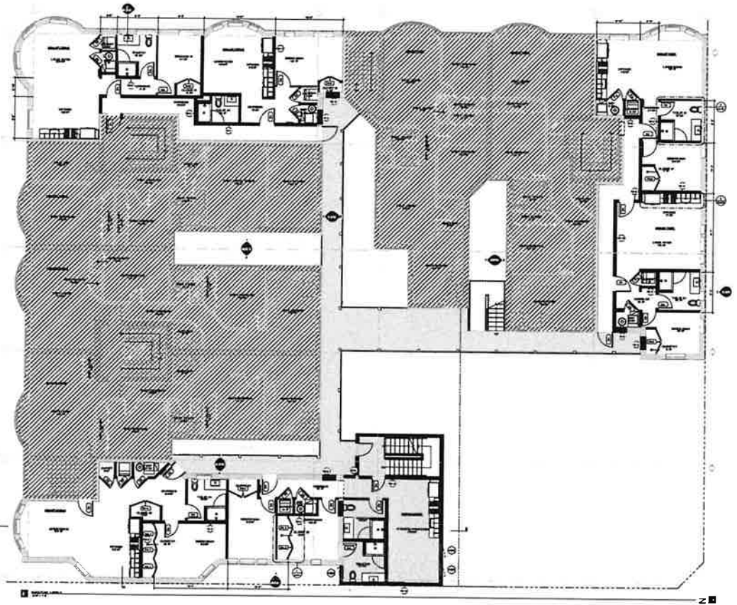
Proposed First Floor Plan (Top) and Second Floor Plan (Bottom) (Source: Future Firm, LLC)
