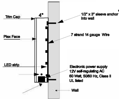
CHANNEL BOX DETAIL (flush mount)
