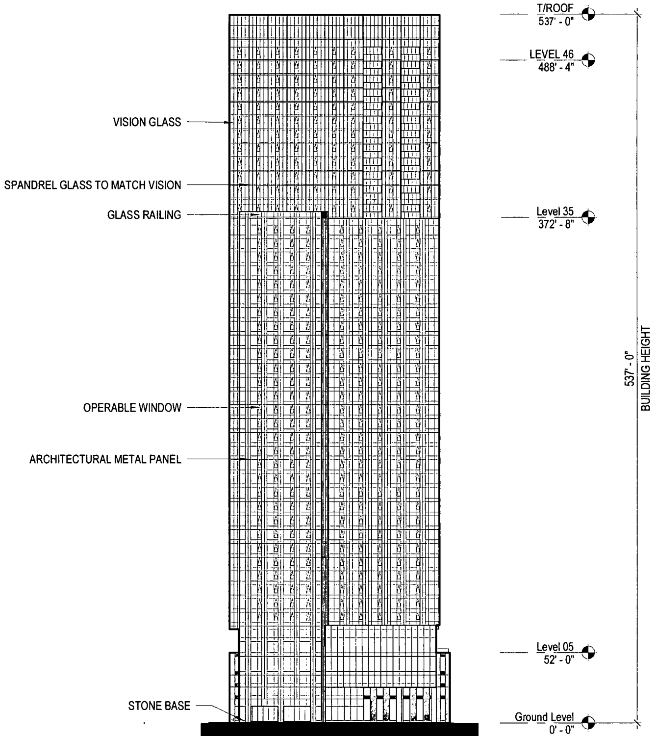
EAST BUILDING ELEVATION Scale: 1" = 50'-0"
