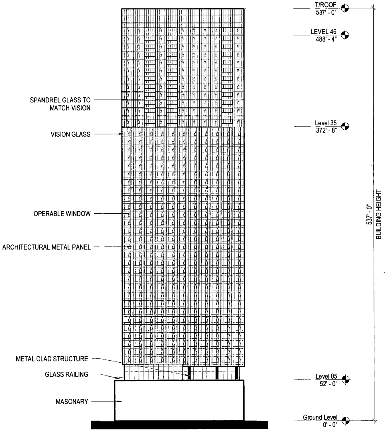
WEST BUILDING ELEVATION Scale: 1" = 50'-0"
