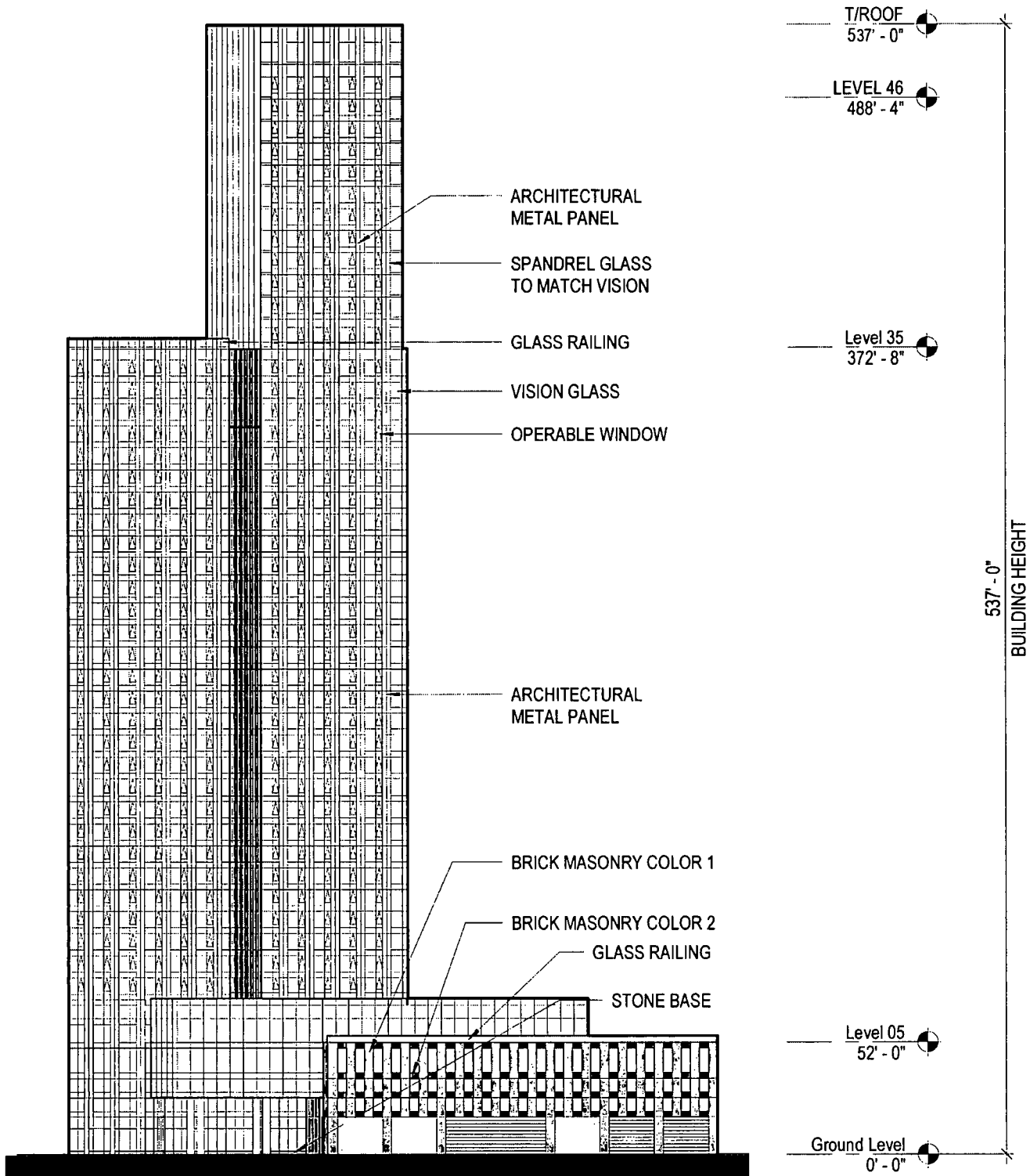
NORTH BUILDING ELEVATION Scale: 1" = 50'-0"
