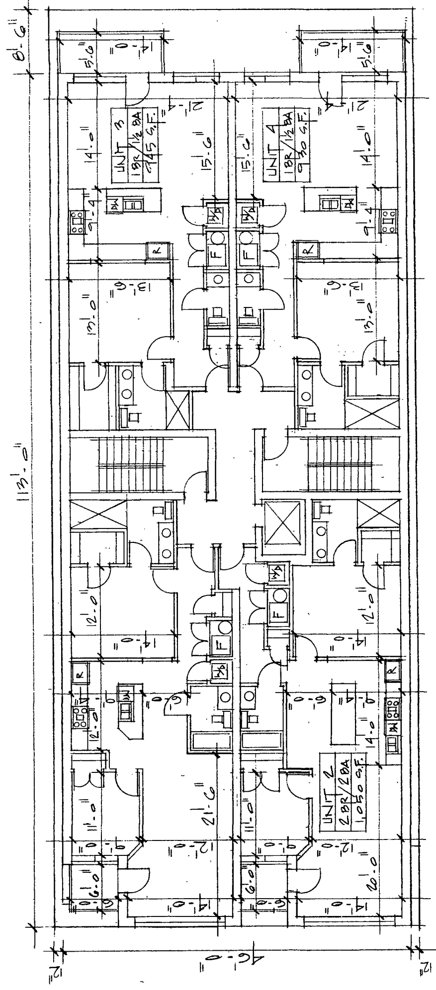
2ND AND 4TH FLOOR PLAN 1/8" = 1'-0"
