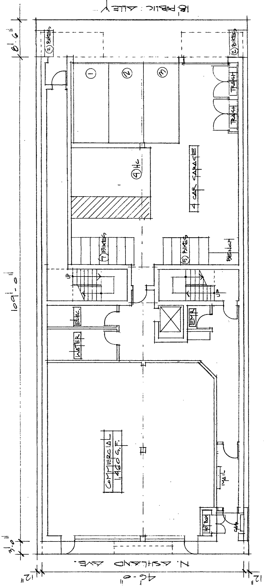
1st Floor Plan 1/8" = 1'-0"
