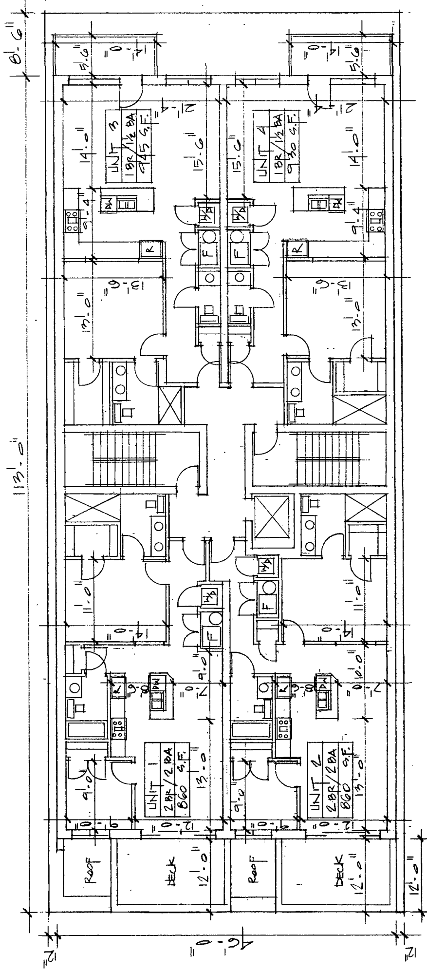
5TH Floor PLAN 1/8" = 1'-0"
