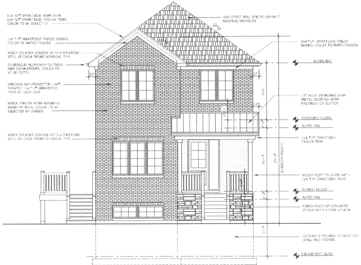
1 FRONT ELEVATION 1/4" = 1'-0"
