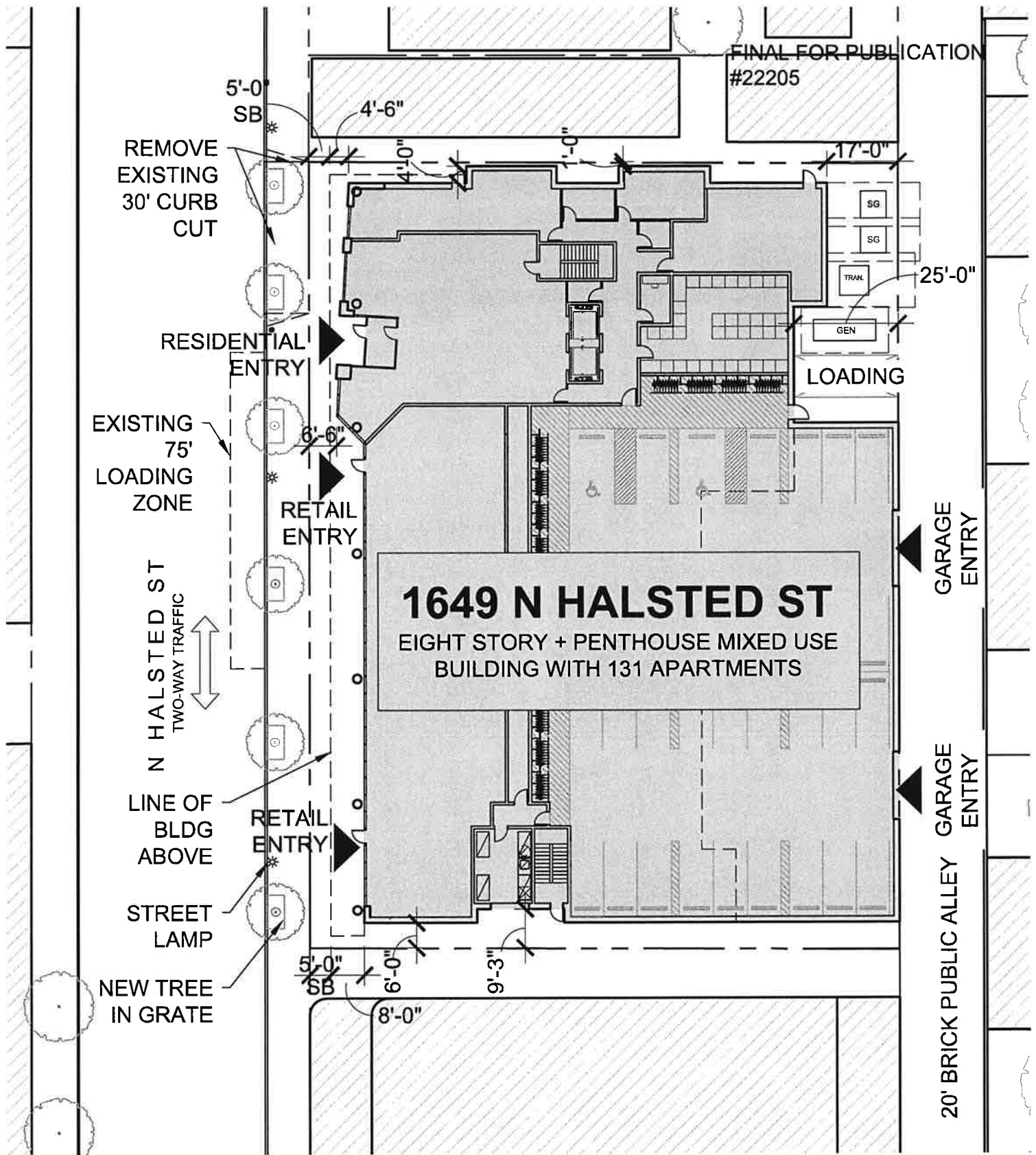
SITE PLAN
